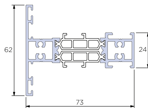
Slim Transom- Screw Fix ACW81.443
