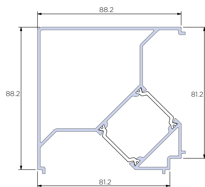
Corner Mullion ACW81.771
