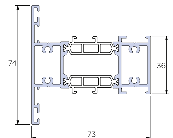
Standard Transom- Screw Fix ACW81.445
