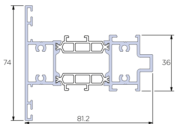
Standard Flush Transom- Screw Fix ACW81.441
