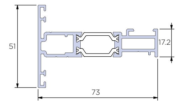
Super Slim Sash ACW81.221
