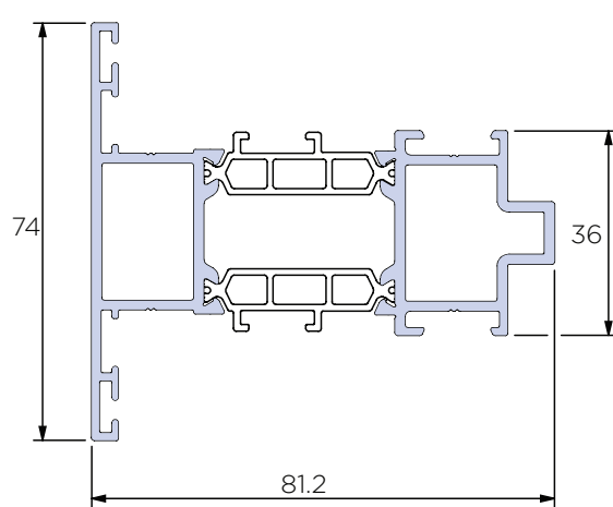
Standard Flush Transom- Cleat Fix ACW81.442
