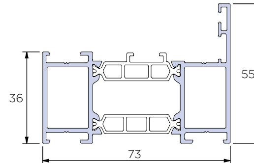
Standard Outer Frame ACW81.114
