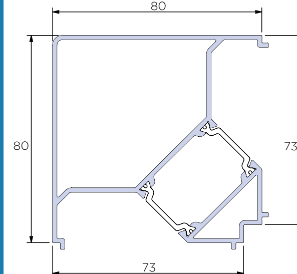
Corner Mullion ACW81.776
