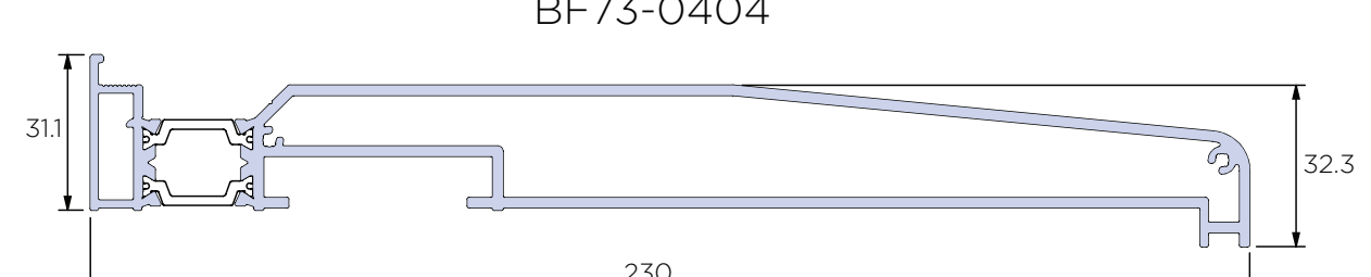
Drainage Sub Cill (230mm) BF73-0404
