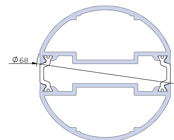
Corner Mullion ACW81.772
