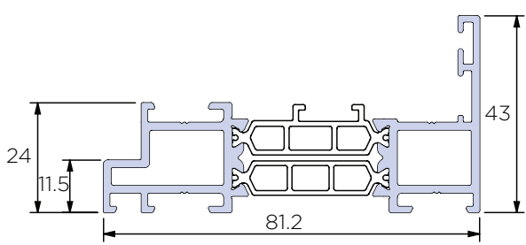
Slim Flush Outer Frame ACW81.111
