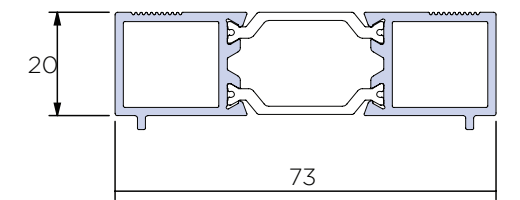
Corner Mullion ACW81.772
