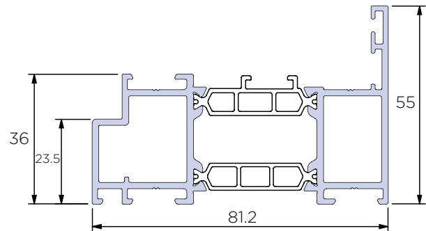
Standard Flush Outer Frame ACW81.112
