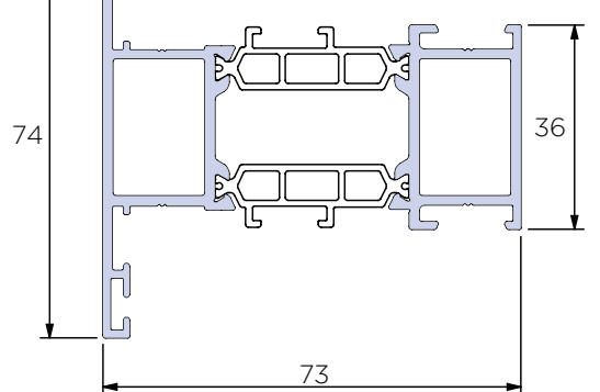
Standard Transom- Cleat Fix ACW81.446
