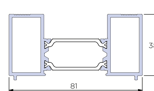
38mm Add on ACW81.662
