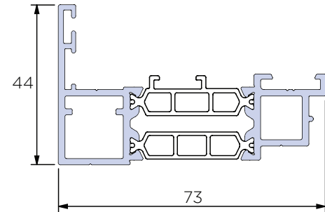
Adaptor ACW81.331
