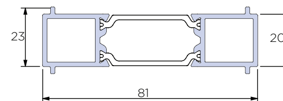
20mm Connector/ 23mm Add on ACW81.661
