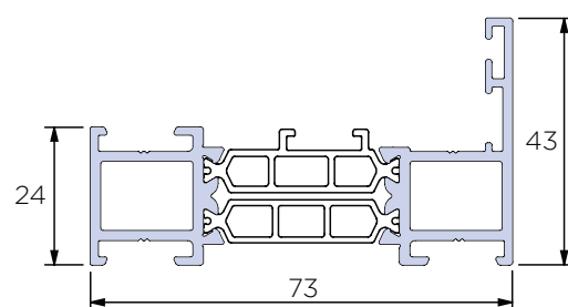
Standard Slim Outer Frame ACW81.113
