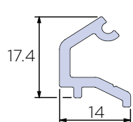
Rotary Clip ACW81.773
