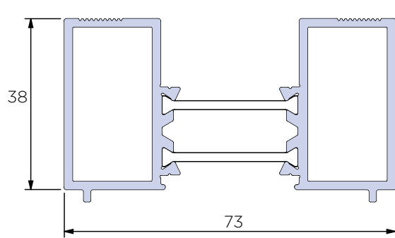
38mm Add on BF73.0503
