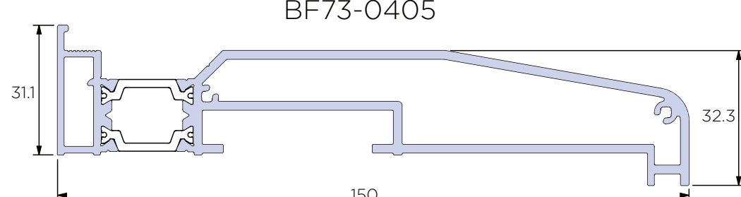
Drainage Sub Cill (150mm) BF73-0405
