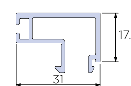
Drainage Sub Cill (190mm) BF73-0403
