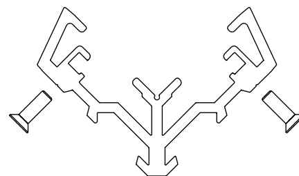
Sash Cleat & Screws BF73.0903K for BF73.0201
