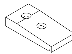
Run Up Block DBA1-204
