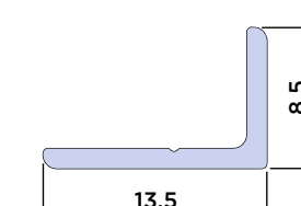
BF73 / WF73 Connecting Profile
