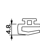
Outer Frame Seal DBA1-144
