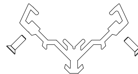
Super Slim Sash Cleat & Screws BF73.0905K for BF73.0203
