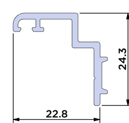
Super Slim Keep Adaptor
