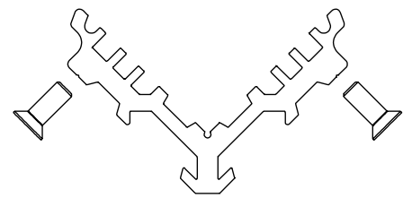
Frame Cleat & Screws BF73.0902K for BF73.0101 & BF73.0102
