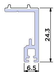
Half Roller Adaptor
