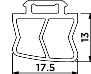
Vertical Sash Seal (13mm) DBA1-145
