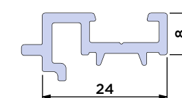
Low Threshold Rebate Add-On
