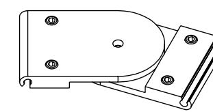
Adjustable Angle Corner Connector DBA1-108 for cills BF73.0401, BF73.0402, BF73.0403, BF73.0404, BF73.0405
