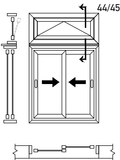
Successive with Opening Sliding or Lift & Slide
