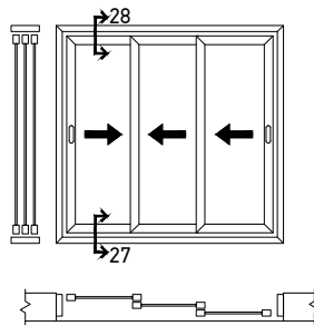
Tree Sash Successive Sliding or Lift & Slide
