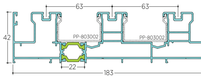
TH 8022 6,5m 3.093 gr/m Triple Rail (Successive)
