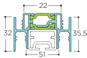
TV 12503 6,5m 119 gr/m Cover for 25mm Interlock TV 12603 & TV 00627 50mm Reinforcement Cover Cap
