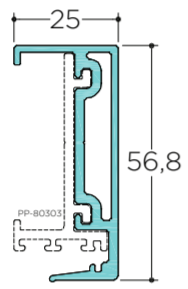
TV 80503 6,0m 133gr/m Clip for Glass Sash
