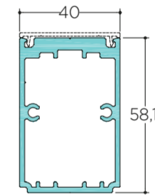
TV 00628 6,5m 1.489 gr/m Reinforcement Profile New Profile for Interlock 50mm
