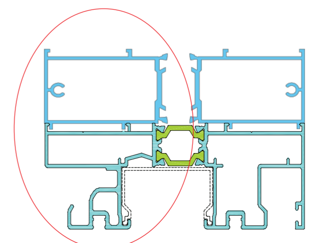
NT-80616 Detail 1 per either side of frame TH80113 or TH8022
