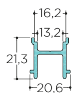
TV 8011 6,0m 279 gr/m Sash Spacer for Lock
