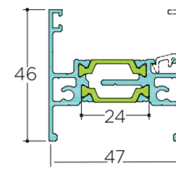
TH 80411 6,5m 1.027 gr/m Interlock Profile 50mm with Clip New Profile for Interlock 50mm
