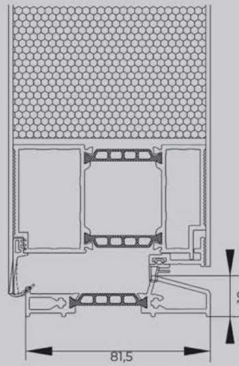
Threshold
